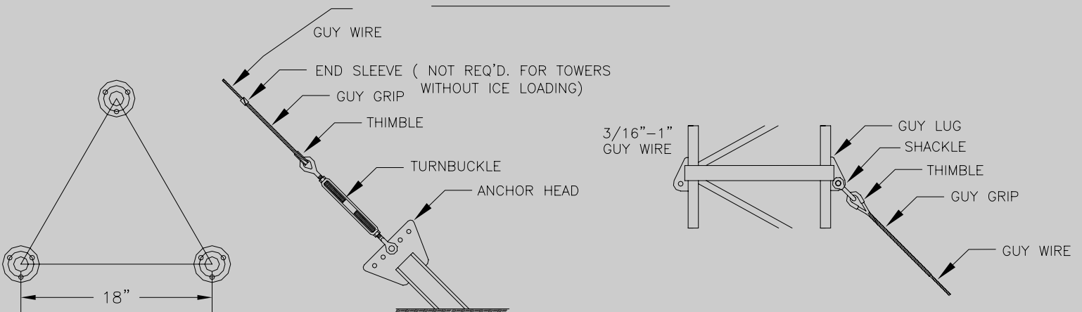
SECTION PLAN
