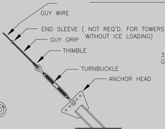
ANCHOR ASSEMBLY
